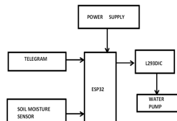
Figure 1: Block Diagram of IoT Based Plant Monitoring System with Telegram Bot
